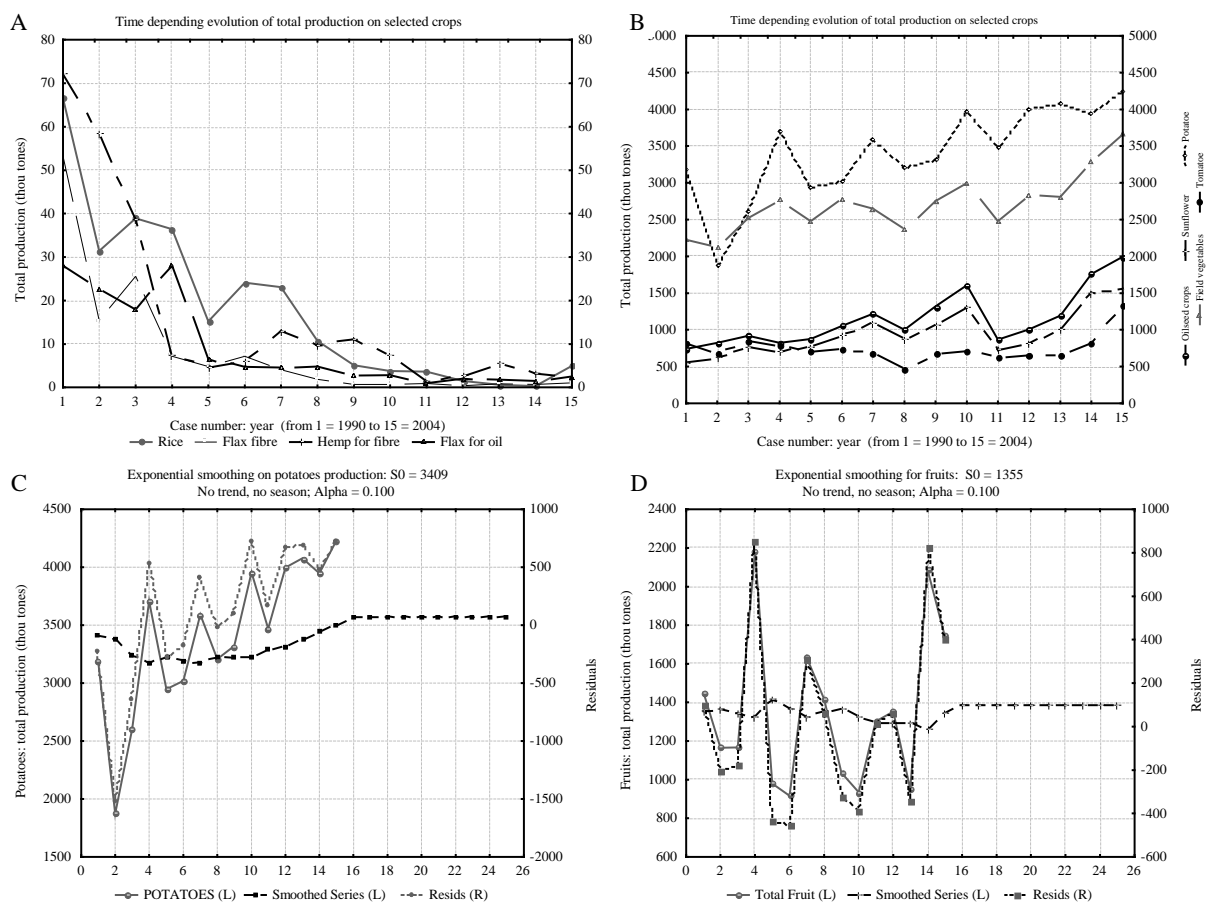
Figure 2. Time series analysis on total production by selected crops: A. Main crops with decreasing production trend; B. Main crops with increasing production trend; C. Exponential smoothing chart on potatoes production; D. Exponential smoothing chart on fruits production
